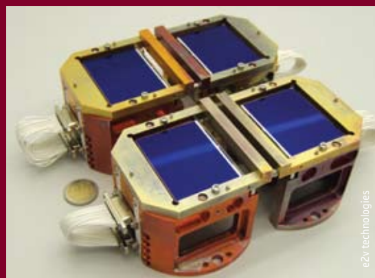
Four of the 106 CCDs that are part of Gaia's large focal plane
