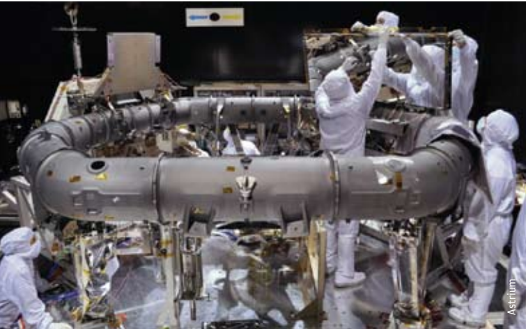
Integration of the first primary mirror on the Payload Module
