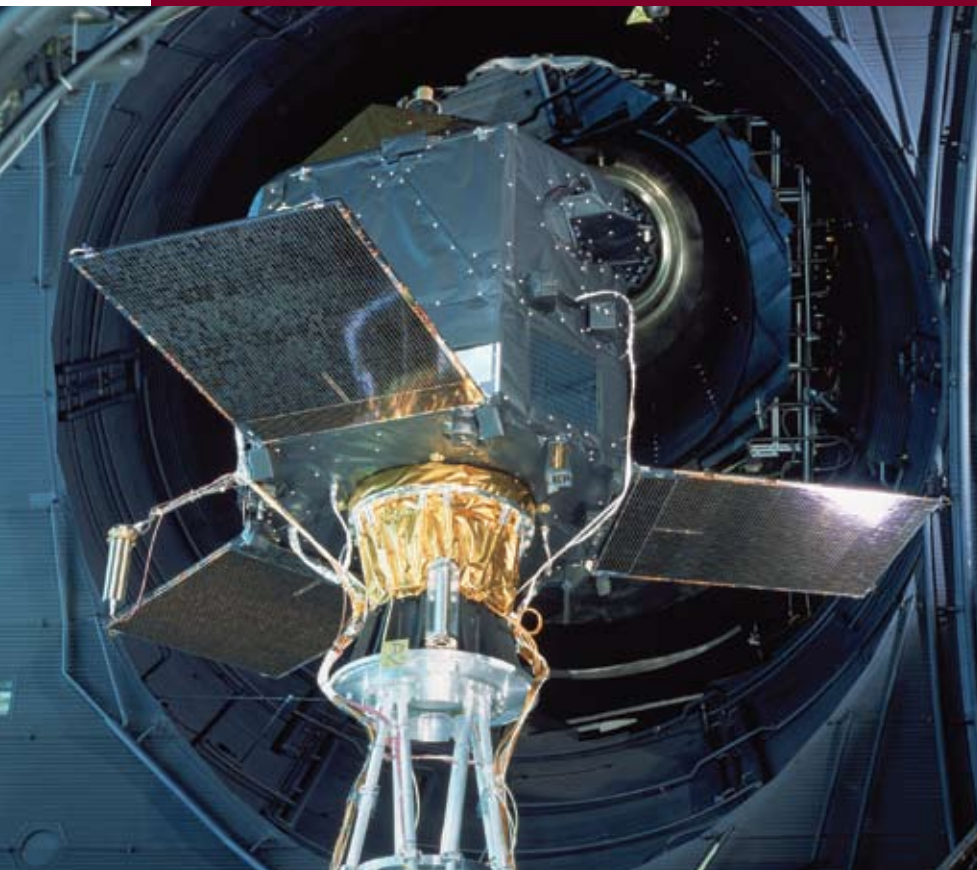
Testing ESA's Hipparcos satellite
