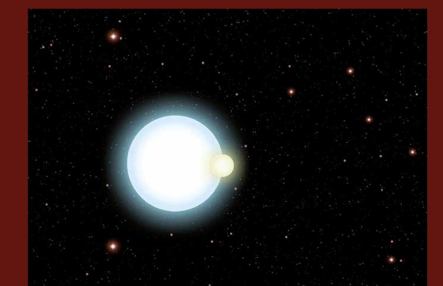
George Foulsham Artist's concept of the binary system NLTT11748 composed of two white dwarfs.
